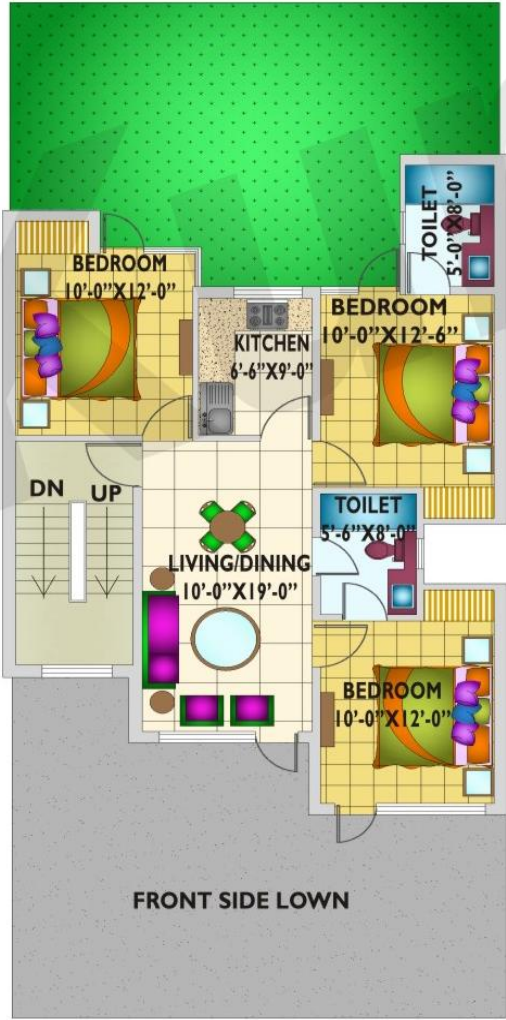
GROUND FLOOR PLAN SUPERAREA 1022 SQFT
